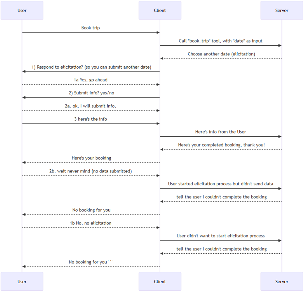
Figure 10.1 – JSON-RPC messages
