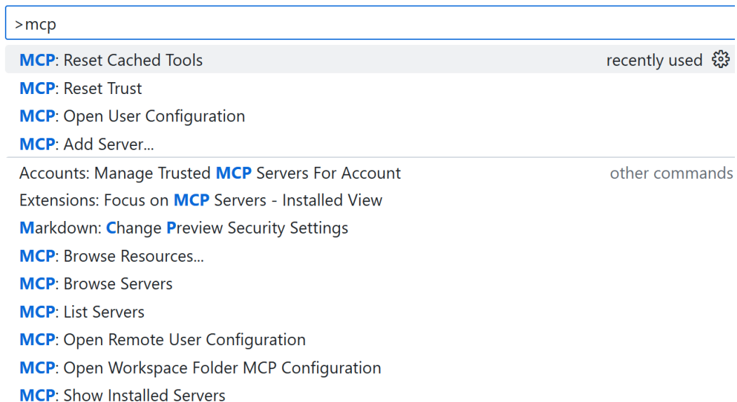
Figure 8.9 – MCP commands
