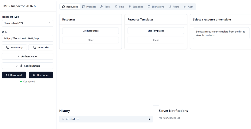
Figure 5.2 – Inspector tool
